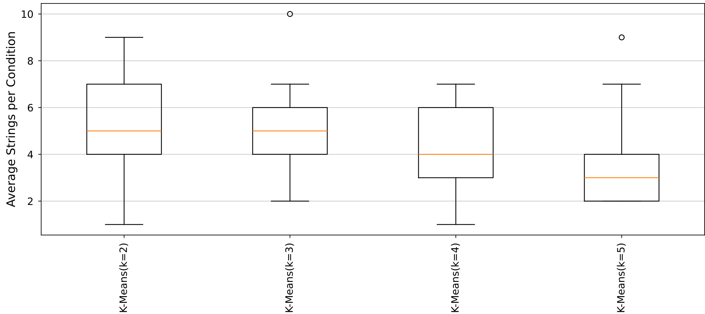
YARA Rules Average Strings per Condition Distribution (Cluster43_Size5 dataset)
